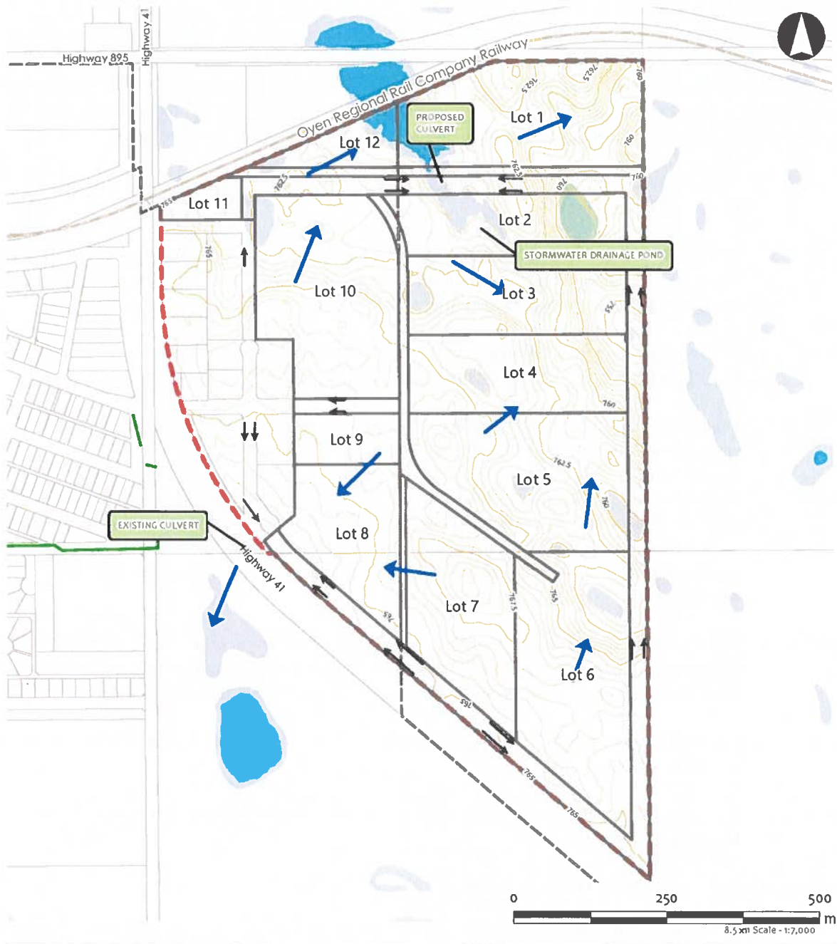
FIGURE 10 | STORMWATER SERVICING
